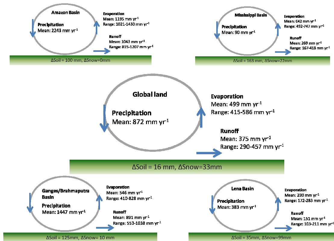
Figure 2.1. Components of water fluxes and storages for terrestrial land surface and four major basins representing different climate regimes, numbers taken from WaterMIP (Haddeland et al. 2011)
