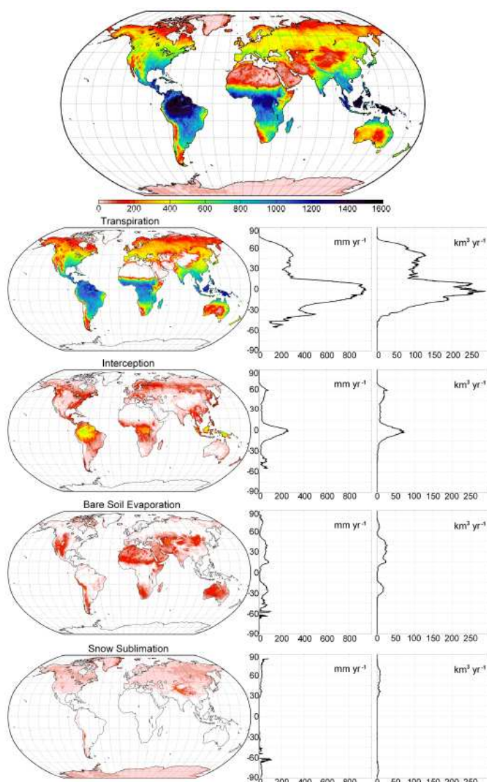
Figure 6.1. Decomposition of 2003-2007 average annual evaporation (mm) into its contributing fluxes. The latitudinal profiles are shown in units of \text{mm yr}^{-1} and \text{km}^3 \text{ yr}^{-1}
