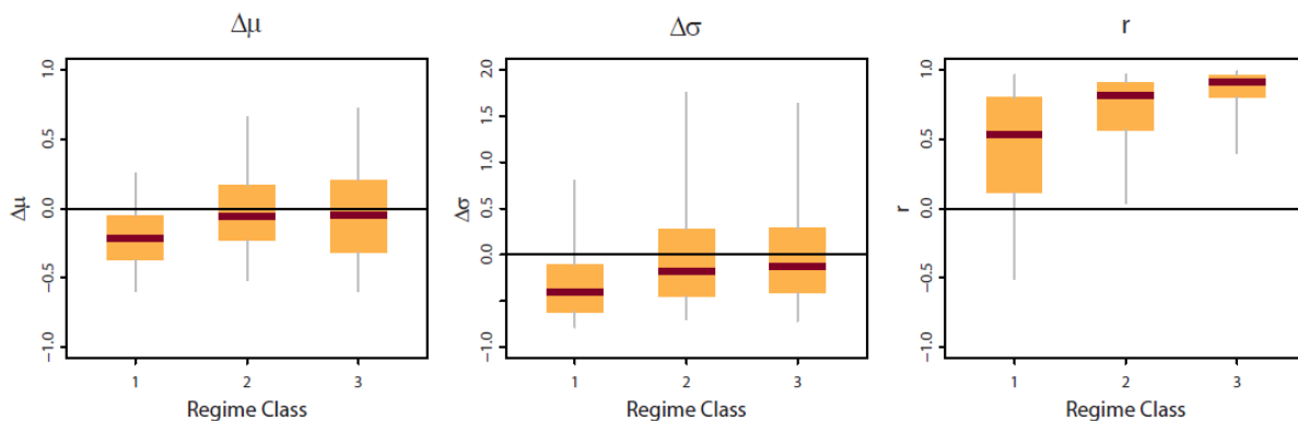
Figure 5.3. Average model performance for each regime-class as measured by the relative difference in mean ( \Delta\mu ), the relative difference in standard deviation ( \Delta\sigma ) and the correlation ( r ). The dark horizontal bar is the median, the box covers the 25 to 75 percentile and the gray whiskers the 5 to 95 percentile.
